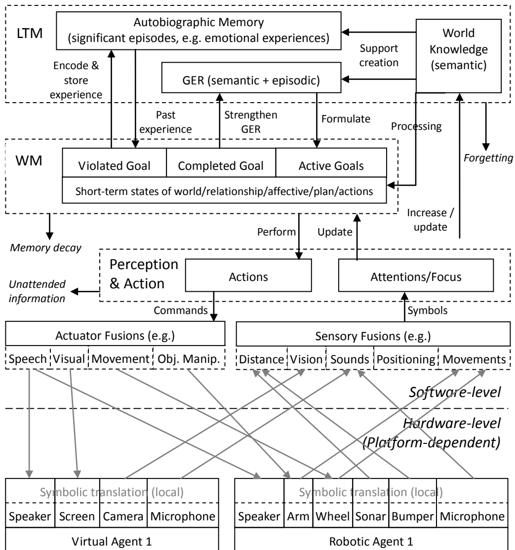
Figure 1: A complete memory model for migrating companion agents, with arrows showing the transition of information among different components. Note that italic labels indicate the effect of forgetting.
